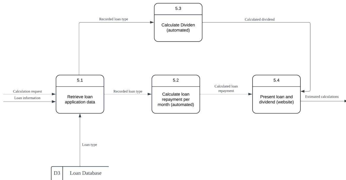
Figure 16: Physical Child Diagram for Process 5
