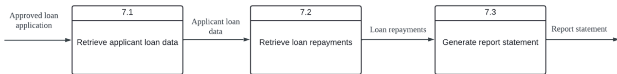
Figure 9: Logical Child Diagram for Process 7
