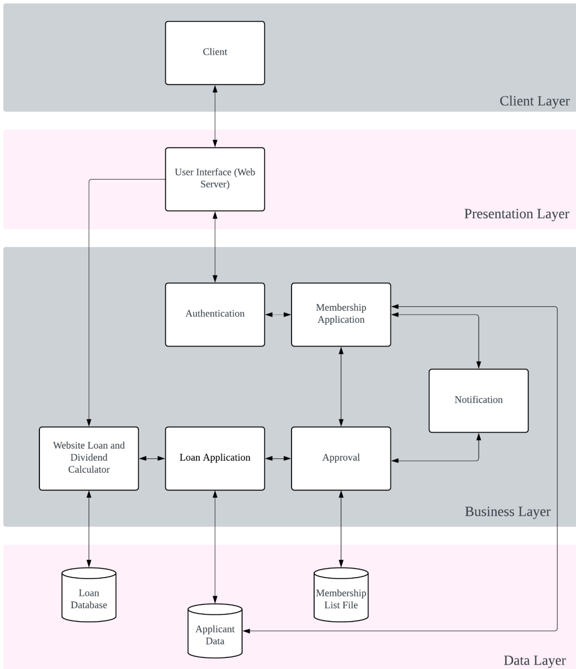
Figure 22: System Architecture
