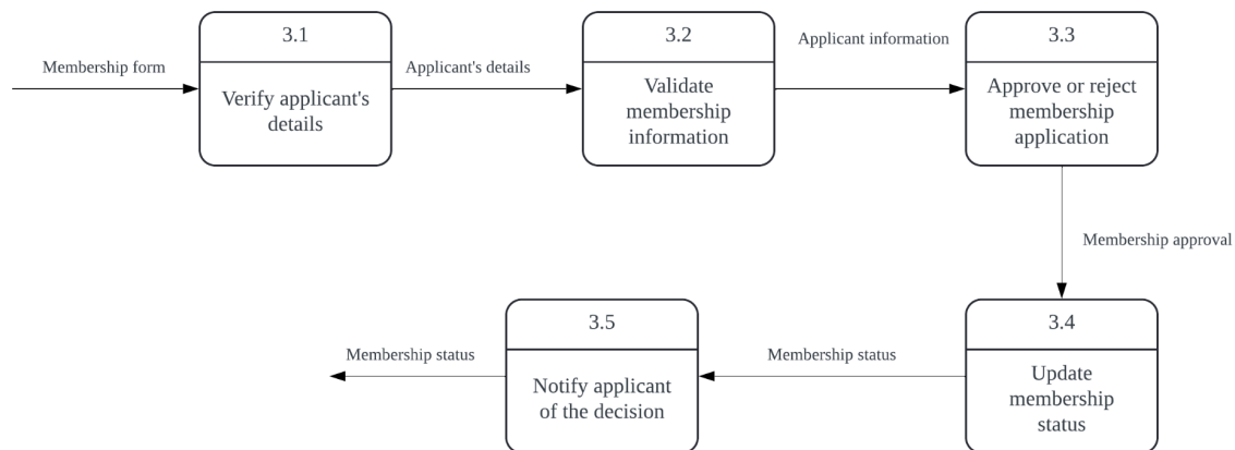
Figure 5: Logical Child Diagram for Process 3
