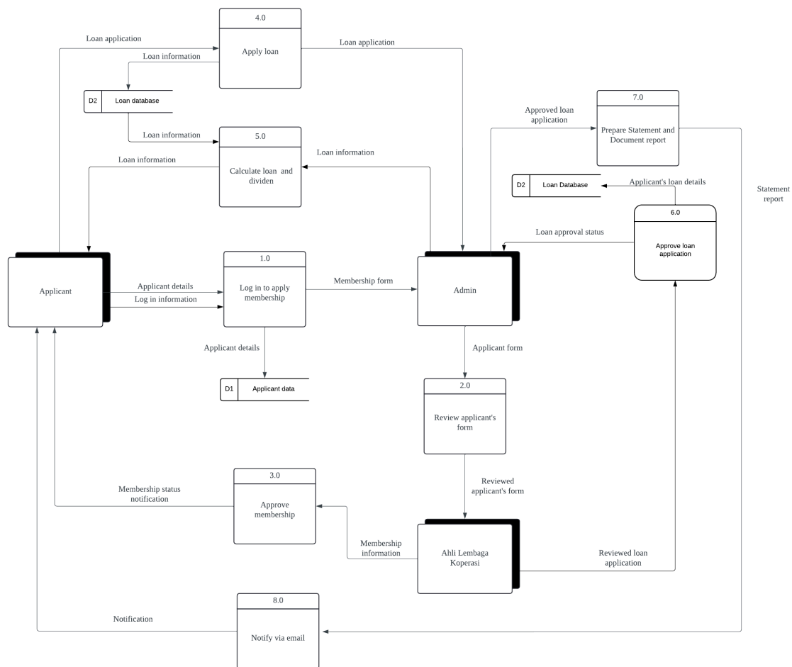
Figure 2: Level 0 Diagram
