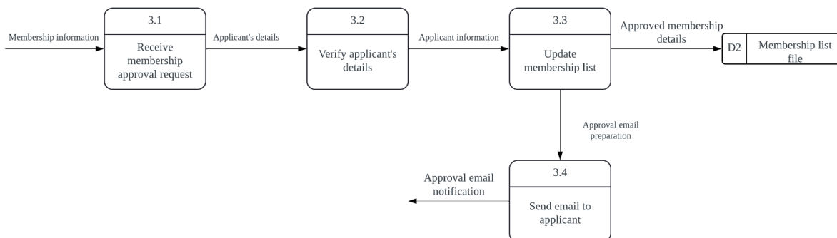
Figure 14: Physical Child Diagram for Process 3
