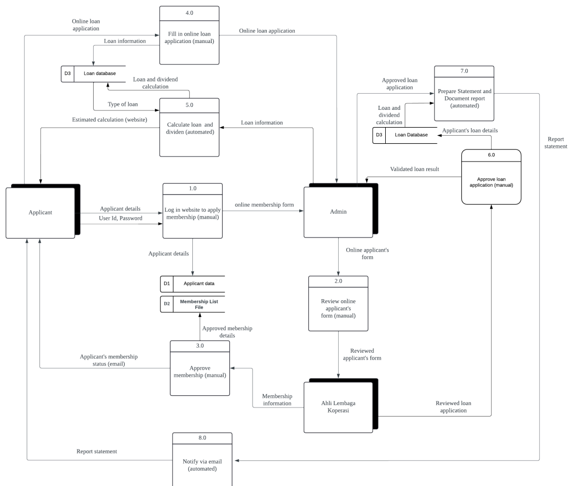
Figure 11: Physical DFD
