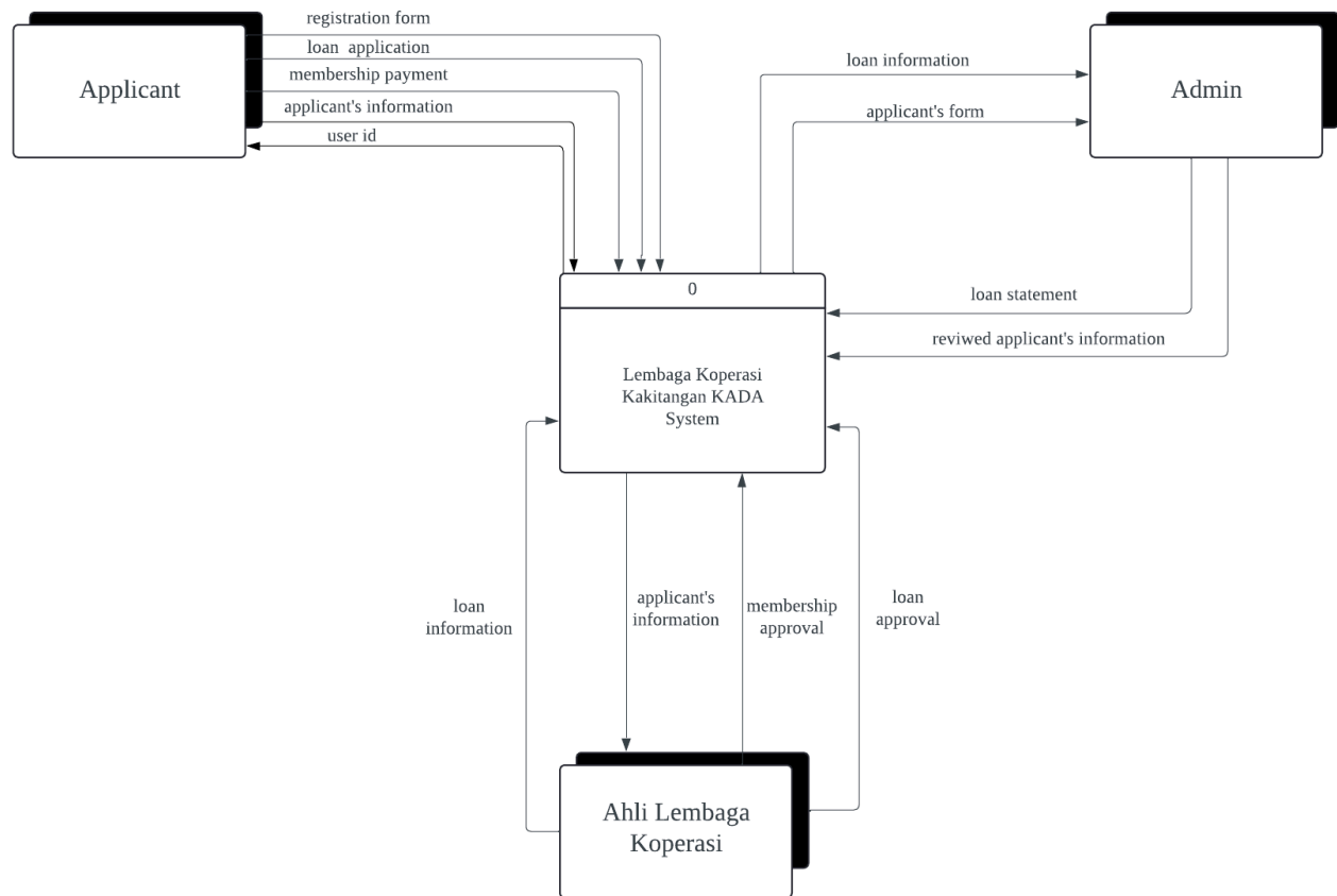
Figure 1: Context Diagram
