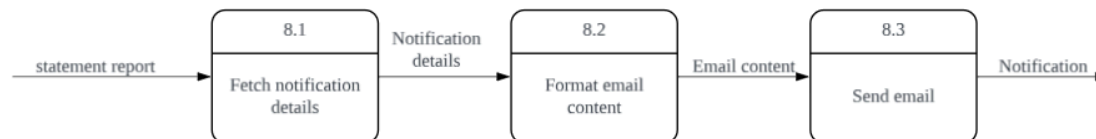
Figure 10: Logical Child Diagram for Process 8
