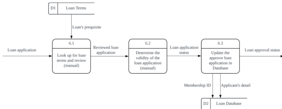
Figure 17: Physical Child Diagram for Process 6
