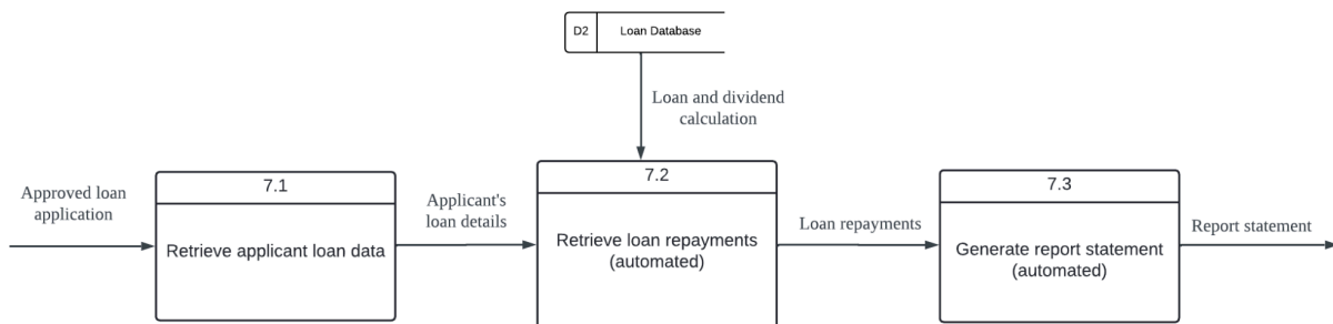
Figure 18: Physical Child Diagram for Process 7
