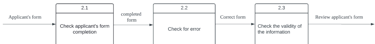
Figure 4: Logical Child Diagram for Process 2
