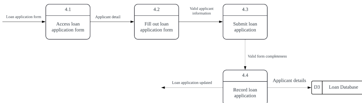
Figure 15: Physical Child Diagram for Process 4
