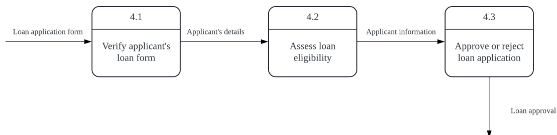
Figure 6: Logical Child Diagram for Process 4
