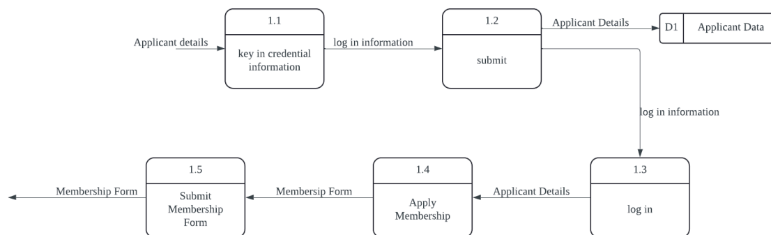
Figure 3: Logical Child Diagram for Process 1
