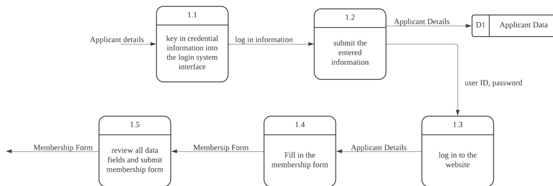
Figure 12: Physical Child Diagram for Process 1
