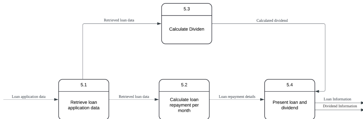
Figure 7: Logical Child Diagram for Process 5
